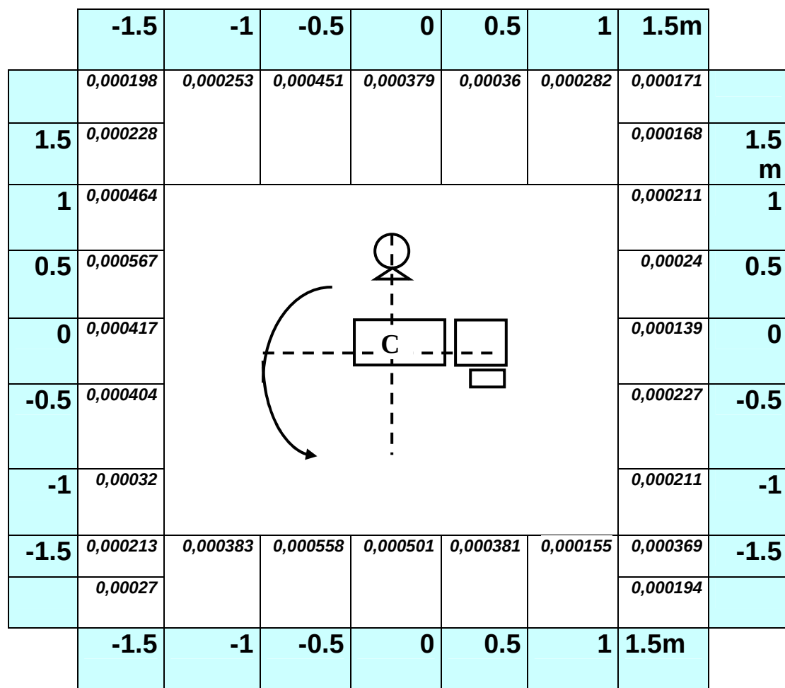
Figure 1: Distribution of scatter radiation
